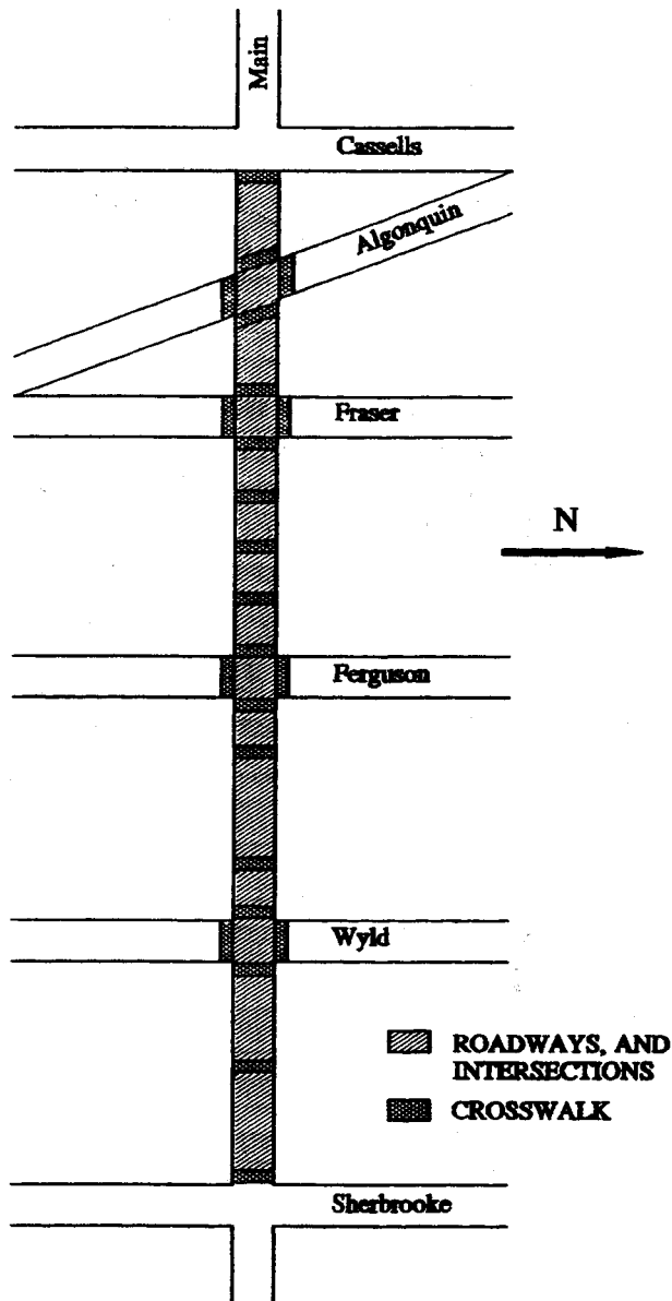
Figure I: Site layout of the reconstruction of Main Street North Bay – 1983 Source: PCS/Law Engineering
